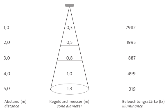
spot 12° + Shutter 19mm (wi4-sh-s)
