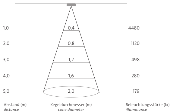
medium 24° + Shutter 38mm (wi4-sh-m)
