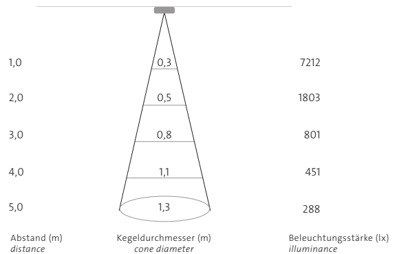
spot 12° + Shutter 76mm (wi4-sh-l)
