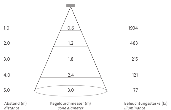
flood 38° + Wabenraster schwarz
