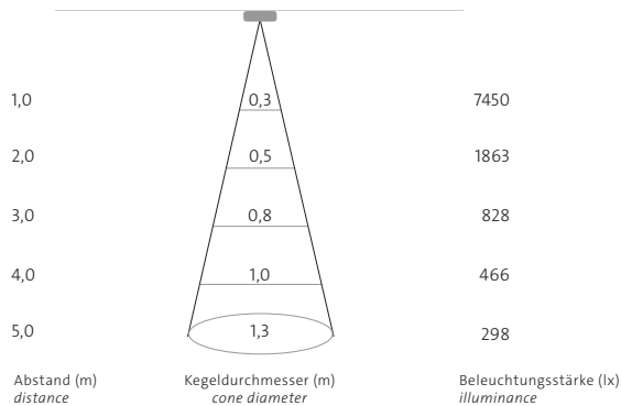
spot 12° + Shutter 38mm (wi4-sh-m)
