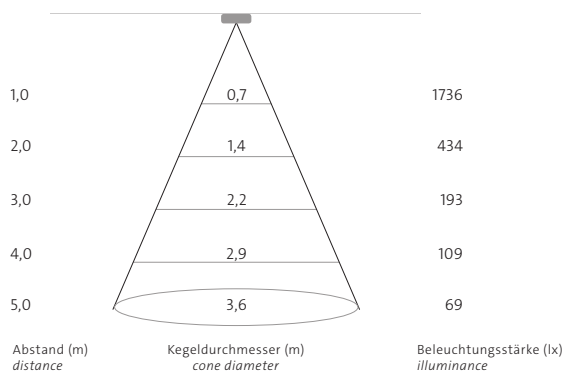
flood 38° + Shutter 38mm (wi4-sh-m)
