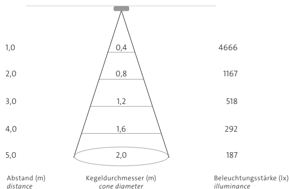
medium 24° + Shutter 19mm (wi4-sh-s)
