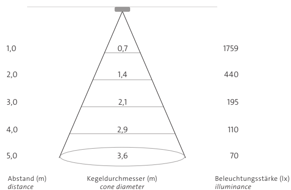
flood 38° + Shutter 19mm (wi4-sh-s)
