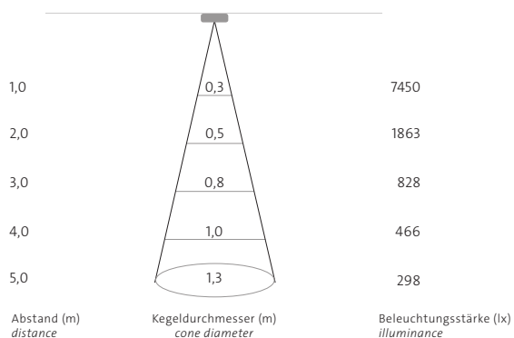
spot 12° + Shutter 38mm (wi4-sh-m)
