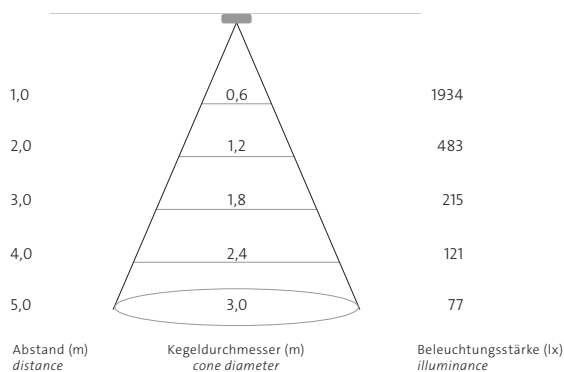
flood 38° + Wabenraster schwarz
