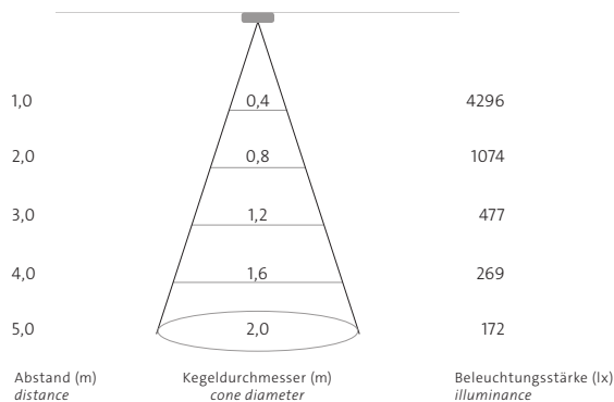
medium 24° + Shutter 76mm (wi4-sh-l)
