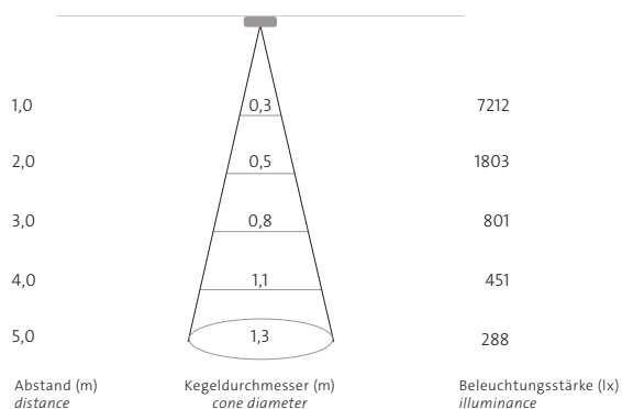
spot 12° + Shutter 76mm (wi4-sh-l)
