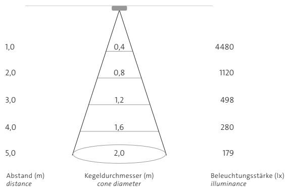
medium 24° + Shutter 38mm (wi4-sh-m)
