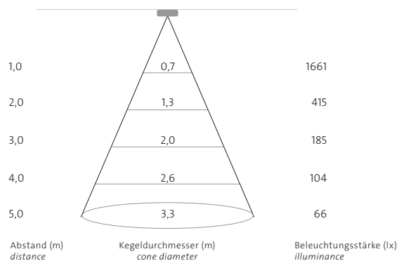
flood 38° + Shutter 76mm (wi4-sh-l)
