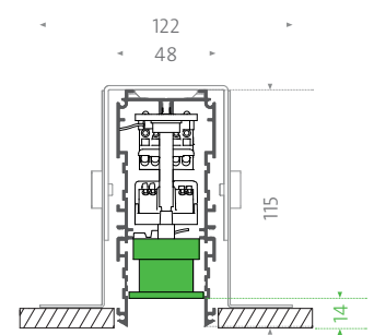
Recessed fbl profile downlight (14 mm) 7/14
