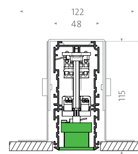
Flush mounted profile with fbl profile downlight 7/14
