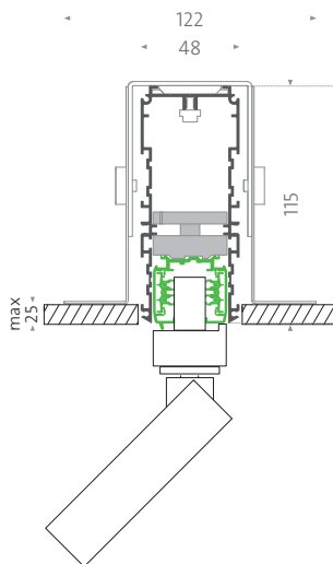
Flush mounted track with fbl-11-7 /-2 + Powergear adapter
