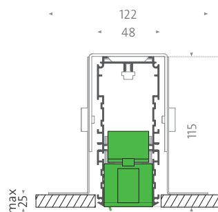
Flush mounted profile with fbl profile downlight for tracks (7/14)
