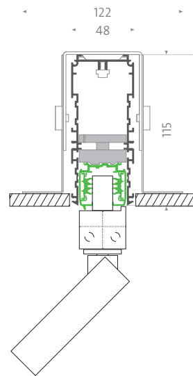
Flush mounted track with fbl-11-4 + Powergear adapter
