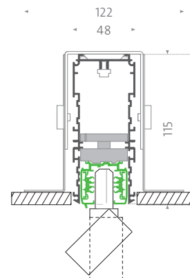
Flush mounted track with fbl-12-in + NPC InviTrack adapter
